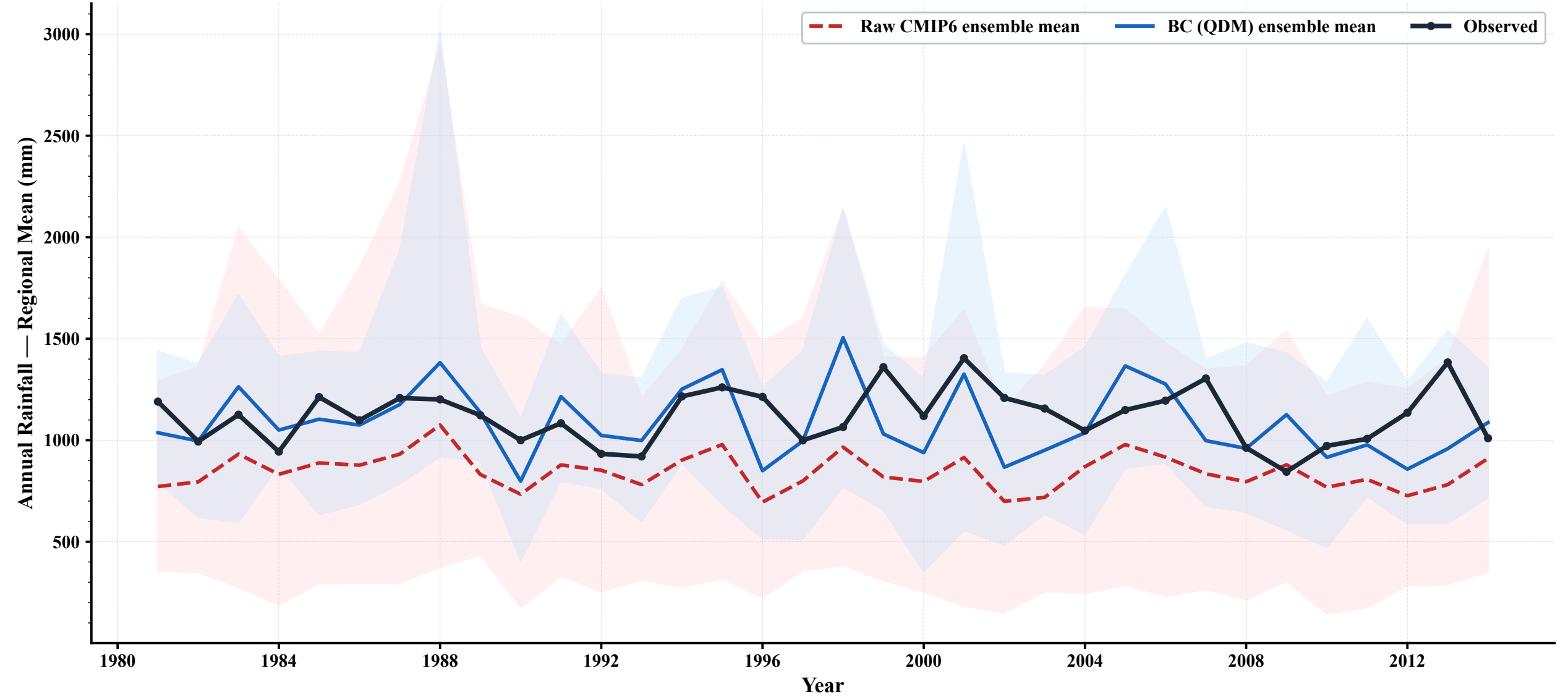
Annual Rainfall Time Series — Regional Mean | 1981–2014 Shaded band = model ensemble range (min–max)
